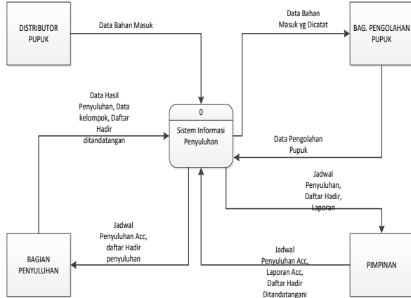
Gambar 2. Context Diagram
