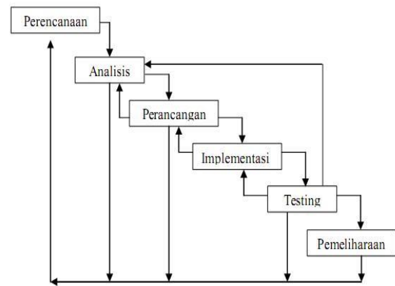
Gambar 1. Metode Waterfall
