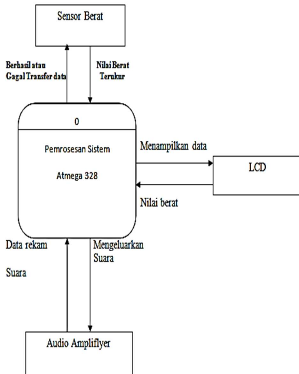
Gambar 3. Context Diagram Sistem
